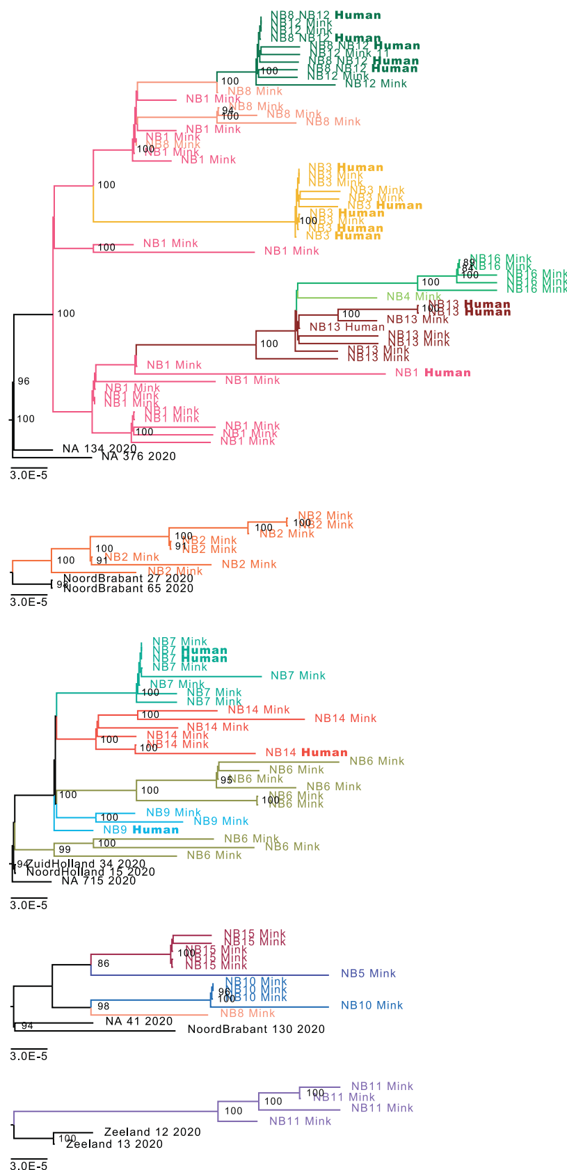
Fig. 3. Phylogenetic analysis of 88 mink and 18 mink-related human SARS-CoV-2 sequences detected in the five mink farm clusters. Sequences derived from different farms are depicted in different colors. The scale bar represents units of substitutions per site.
